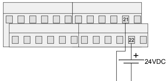
Gangreserve-Batterie ETC 12/14/24
